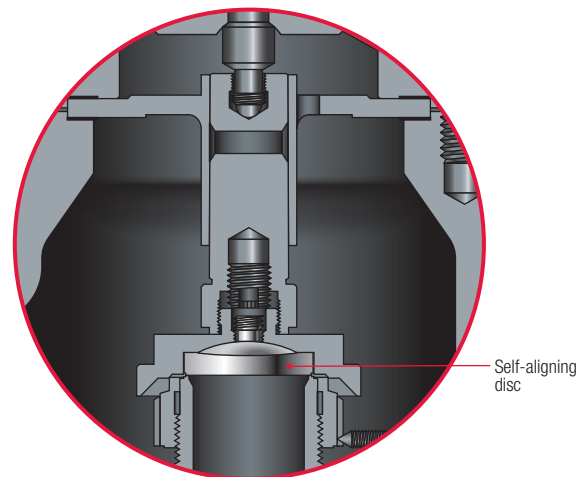
High Strength Disc Figure No. 6
