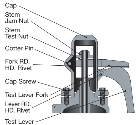
Open Lever (Double Acting Lever) Sizes 1x2 Thru 6x10 Except #150 and #300LW, Sizes 8x10, All Types
