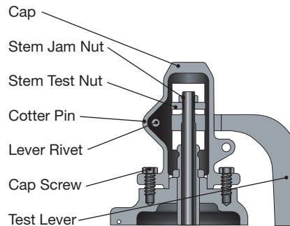
Open Lever (Single Acting Lever) #150 and #300LW, All Sizes Except 8x10
